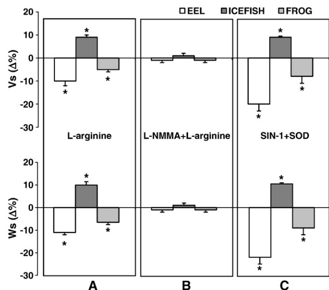
Fig. 2. Effect of L-arginine on stroke volume (Vs) and stroke work (Ws) in isolated and perfused hearts of eel ( 10^{-7} mol l^{-1} ), icefish ( 10^{-6} mol l^{-1} ) and frog ( 10^{-7} mol l^{-1} ) before (A) and after (B) treatment with L-NMMA ( 10^{-5} mol l^{-1} ) ( n=4-7 ). (C) Effect of SIN-1 (in presence of SOD 10 IU/ml) on stroke volume (Vs) and stroke work (Ws) in eel ( 10^{-7} mol l^{-1} ), icefish ( 10^{-5} mol l^{-1} ) and frog ( 10^{-7} mol l^{-1} ) ( n=4-5 ). Percentage changes were evaluated as means \pm S.E.M. Asterisks indicate values significantly different from the control value: * P<0.05 .
